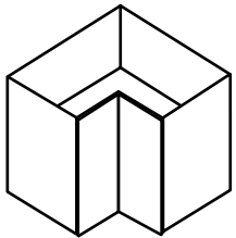
Corner base cabinet 900 x 900mm
